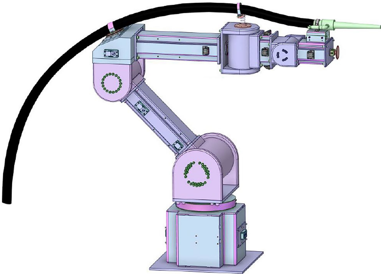
Figure 1 — Full overview of SFR robotic manipulator, including hose management system and actuated tool
