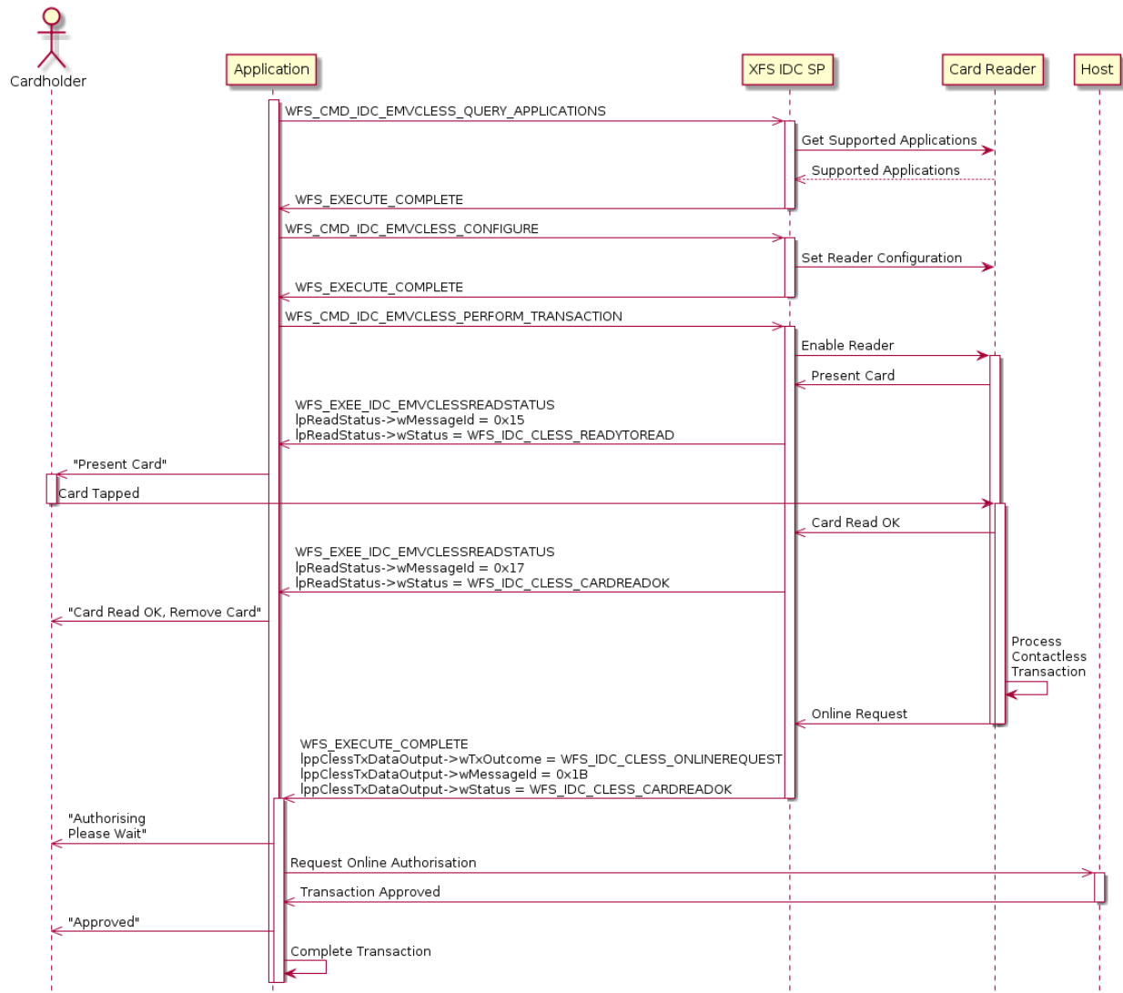
Figure 1 - Single tap transaction with no issuer update data received from host
