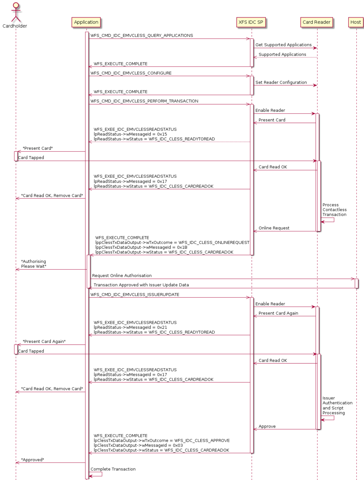
Figure 2 - Double tap transaction with issuer update data received from host
